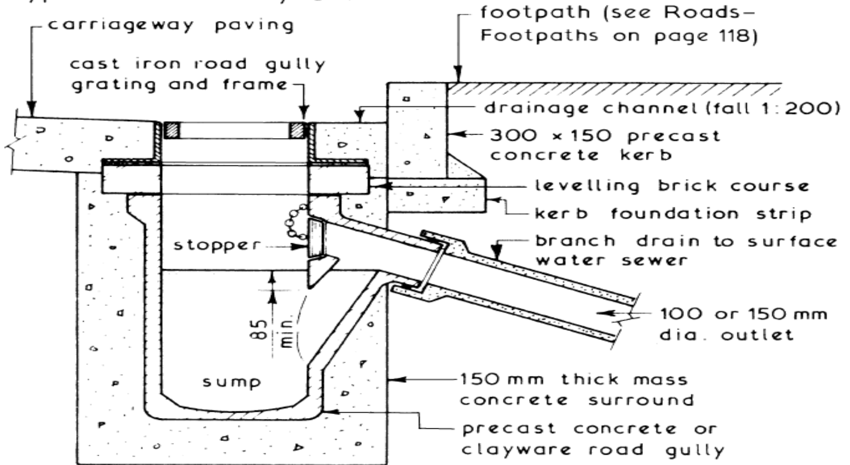
Typical Road Gully Detail ~
