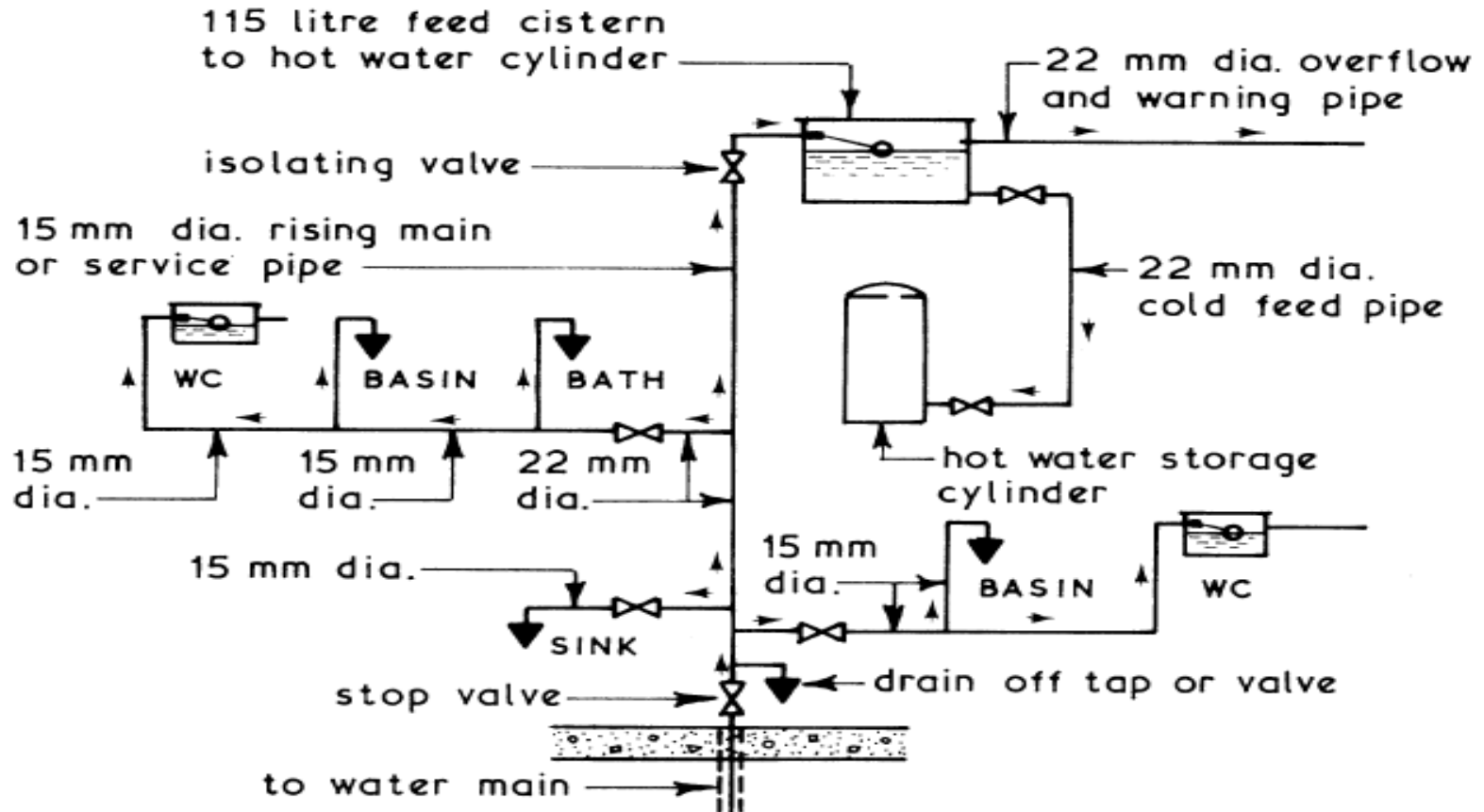
Typical Direct Cold Water System ~
