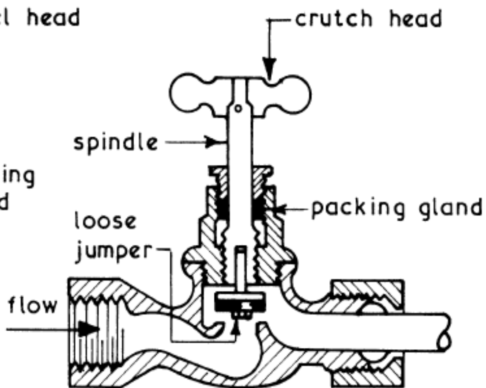
STOP VALVE
