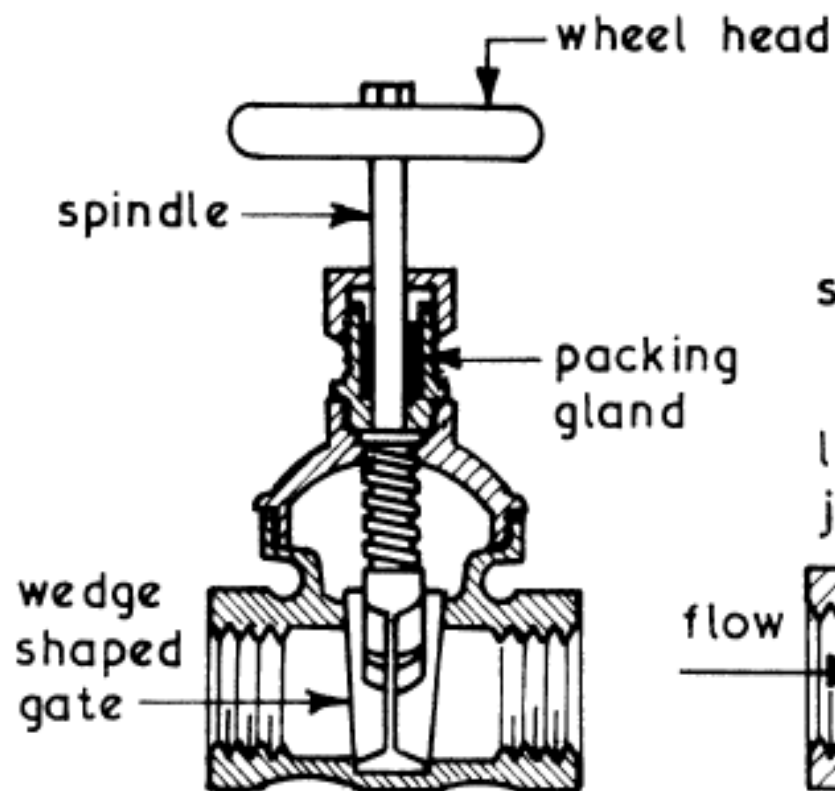
GATE VALVE
