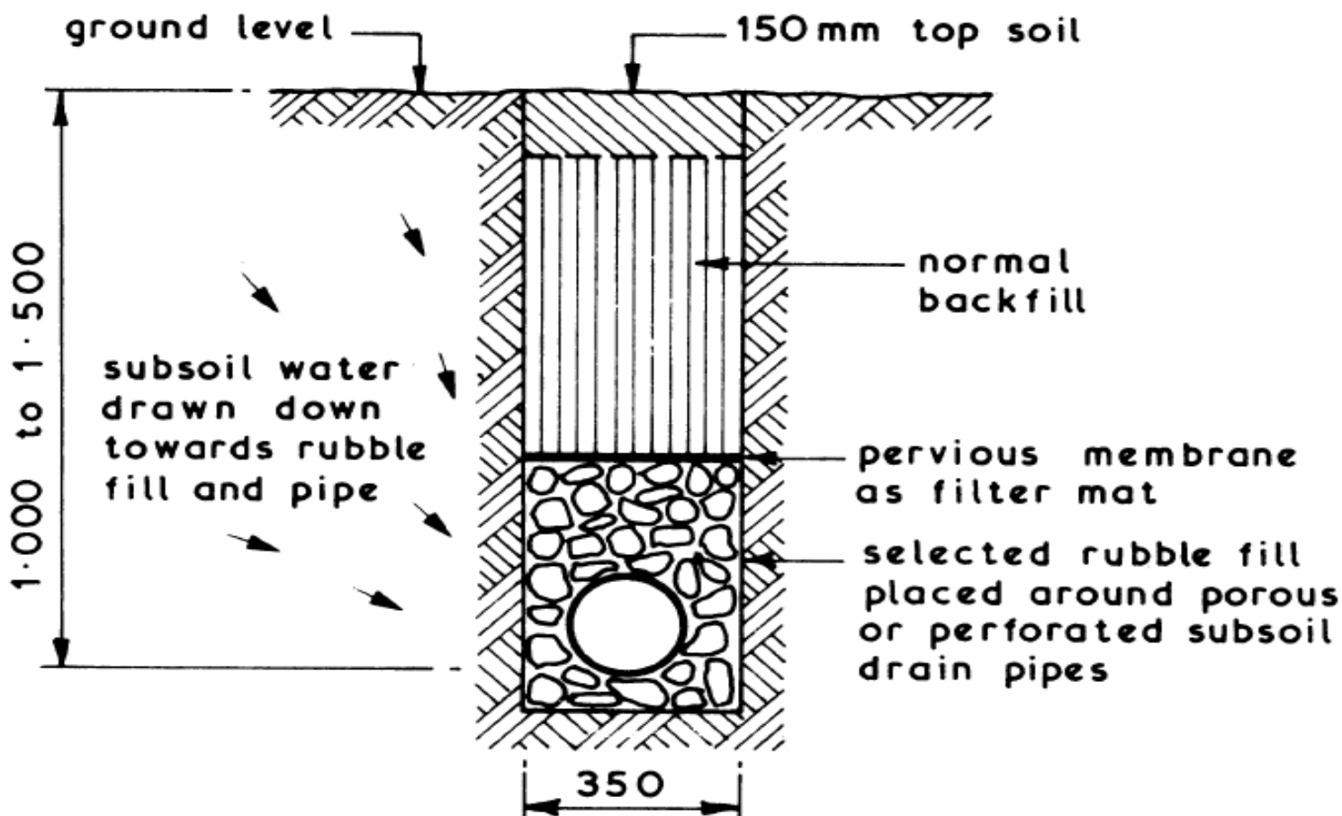
Typical Subsoil Drain Details ~
